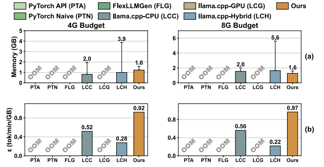
Figure 10: Performance on dynamic memory budgets.
