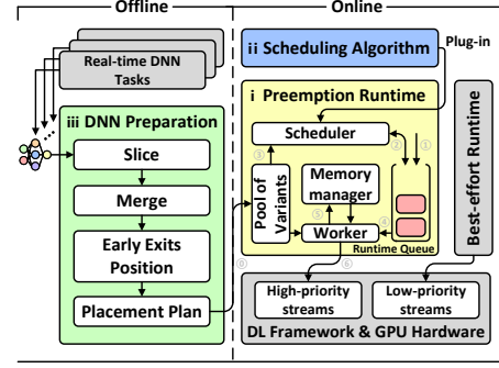
Figure 2: Overview of the Pantheon design.
