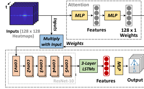
Figure 10: Skeleton tracker design, which reads heatmaps as input to estimate the 3D coordinates of 19 skeleton points.
