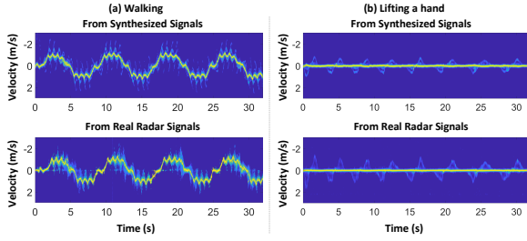
Figure 6: For two activities (a) walking and (b) lifting a hand, the 1 st row shows the micro-Doppler spectrum derived from our synthesized signal, and the 2 nd row shows the corresponding micro-Doppler spectrum from real mmWaves.
