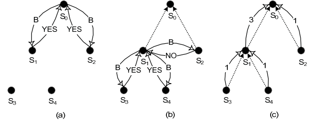
Figure 4 An example of network initialization in RPS-LB-D
