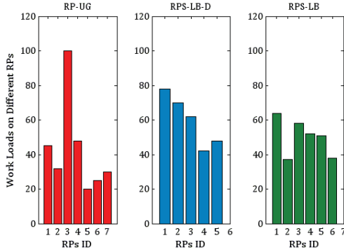
Figure 8 Workloads on the RPs in different algorithms.
