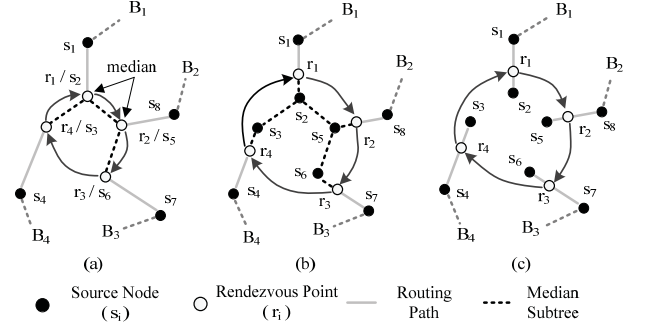
Figure 3 An example of the RPS-LB algorithm's execution. (a) T_m after the first iteration. (b) The final T_m is of size Y . (c) The final solution.
