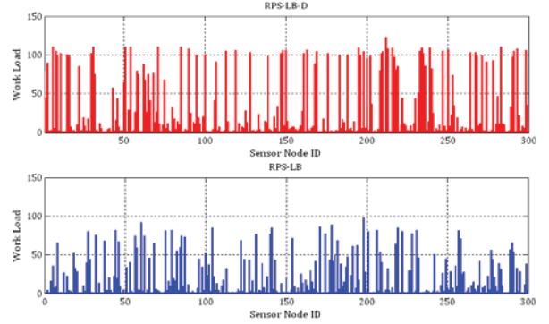
Figure 9 Workloads on sensor nodes in RPS-LB-D and RPS-LB.
