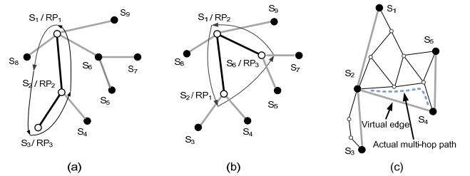
Figure 1 (a) Trajectory planning produced by the simple greedy strategy. (b) Trajectory planning with the workload balancing. (c) Underlying network topology and the geometrically approximated routing tree. The network topology is represented by black lines and hollow circles. The routing tree is represented by grey lines and solid circles.
