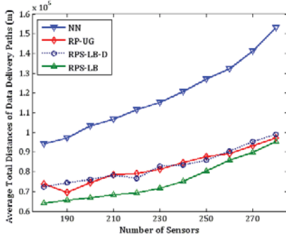
Figure 5 Total distances of data delivery paths vs. Number of source nodes.
