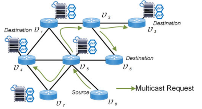
Fig. 1. An MEC network G .
