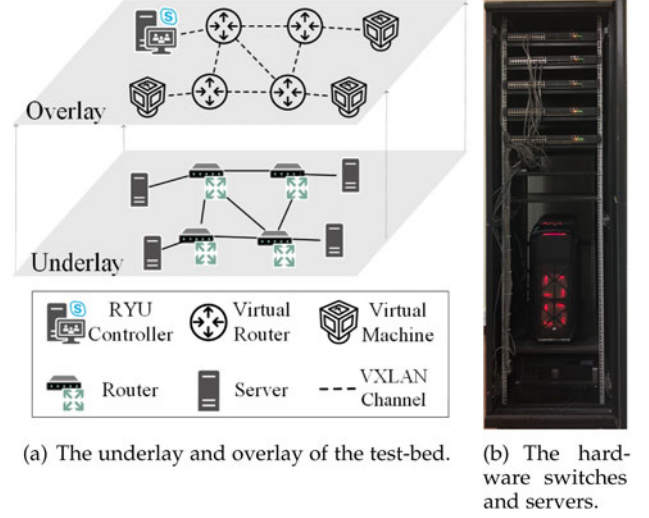
Fig. 8. A test-bed with both hardware switches and virtual resources.
