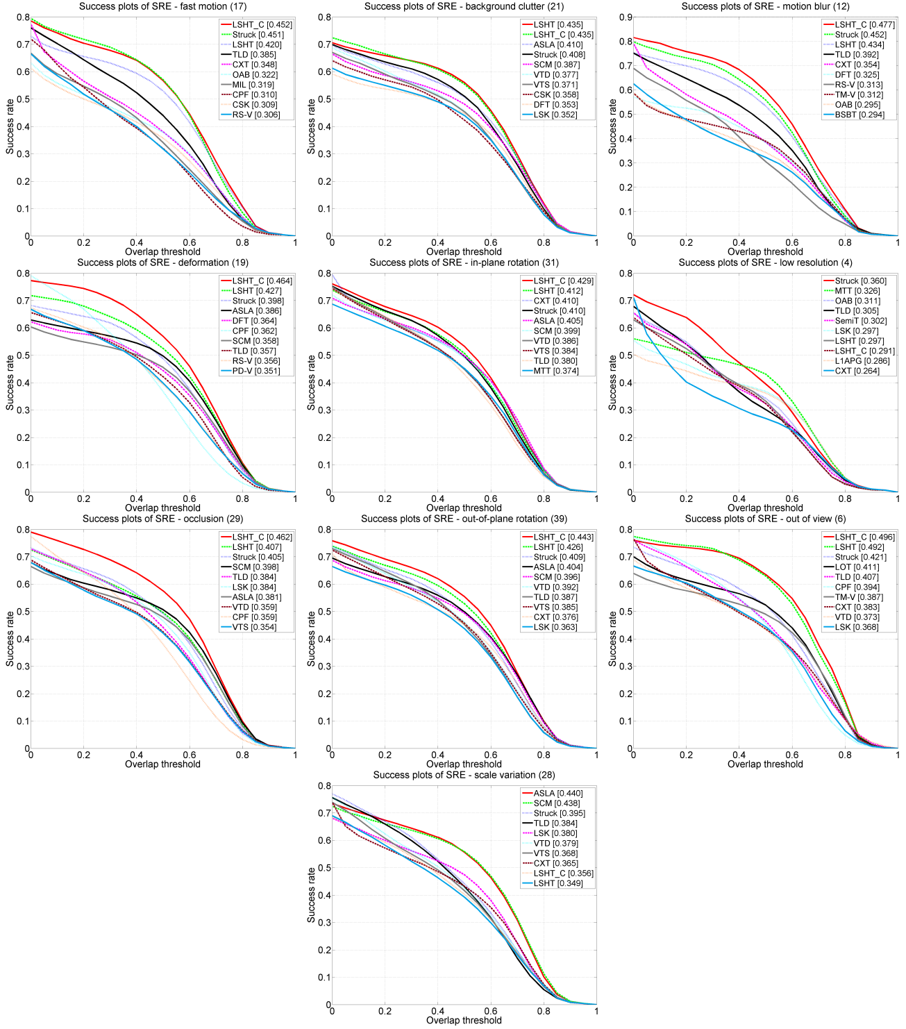
Fig. 4: The SRE plots under 10 challenging factors. The average AUC scores are shown in the legends.
