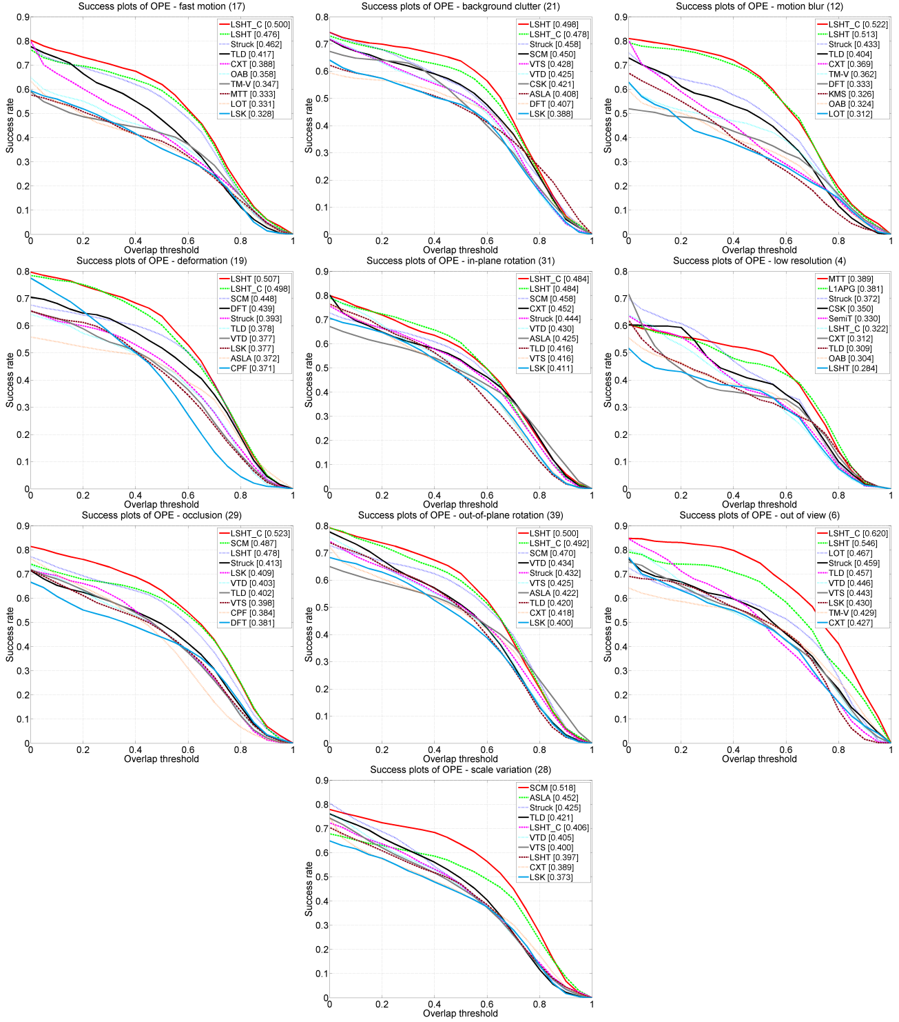
Fig. 2: The OPE plots under 10 challenging factors. The average AUC scores are shown in the legends.
