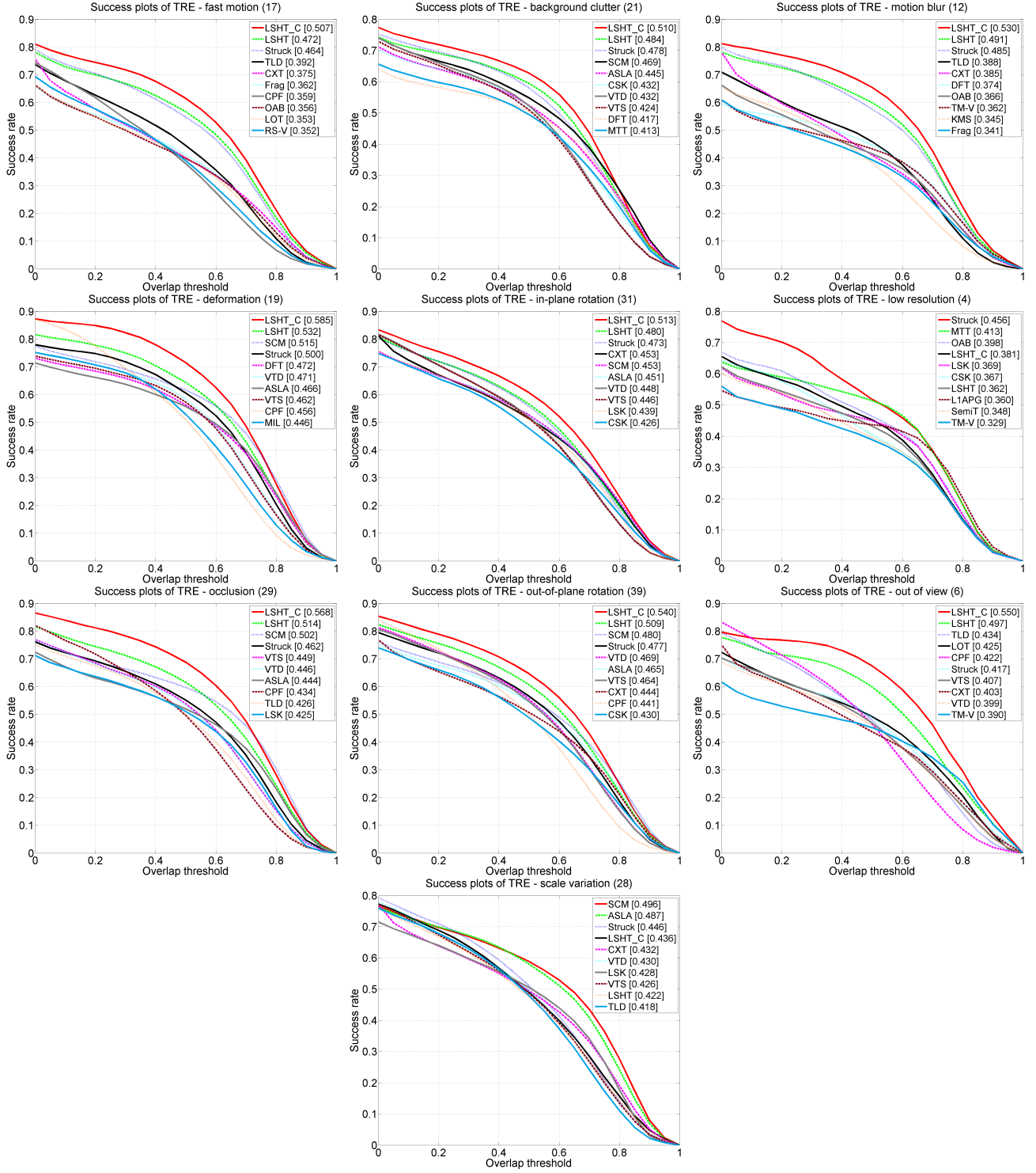
Fig. 3: The TRE plots under 10 challenging factors. The average AUC scores are shown in the legends.
