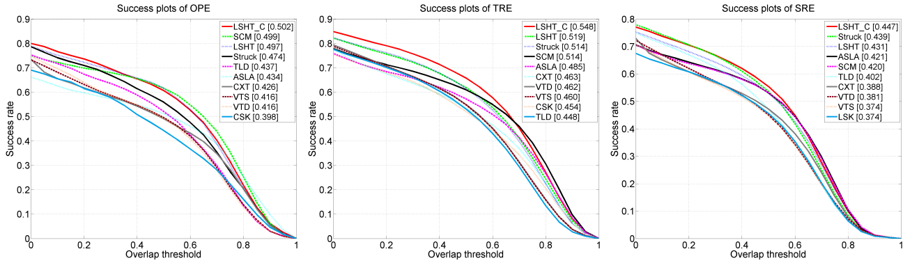
Fig. 1: Overall performances using three different metrics OPE , TRE , and SRE . The average AUC scores are shown in the legends.
