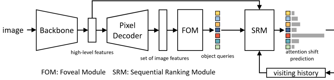
Figure 2: SeqRank is composed of a backbone network, a pixel decoder, a Fovea Module (FOM), and a Sequential Ranking Module (SRM). The FOM learns to progressively refine the learnable object queries from image features, while the SRM predicts the next object that is likely to be visited, conditioning on the previous visiting history. By continuously updating the visiting history and invoking the SRM, all salient objects can be detected in a sequential order that reflects how human attention shifts among them.
