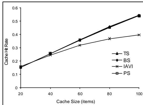
Figure 8: Cache Hit Rate vs Cache Size
