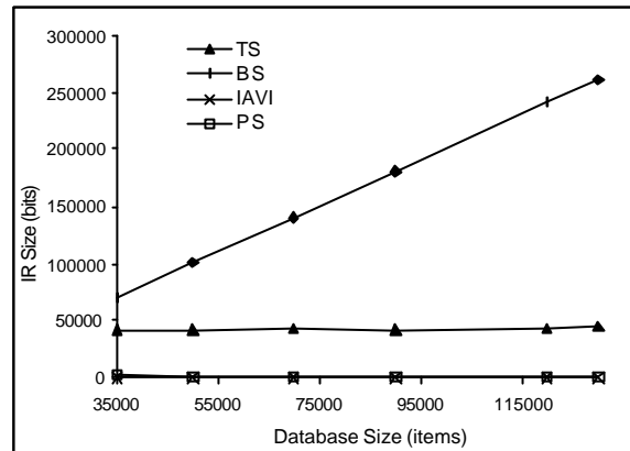
Figure 4: Invalidation Report Size vs Database Size
