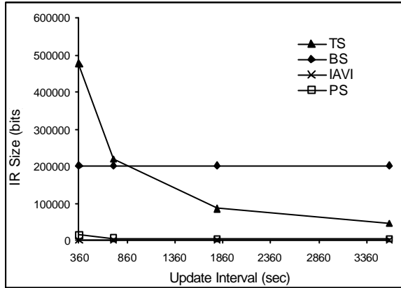
Figure 6: Invalidation Report Size vs Update Interval
