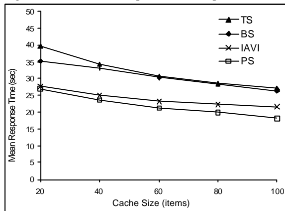
Figure 7: Mean Response Time vs Cache Size
