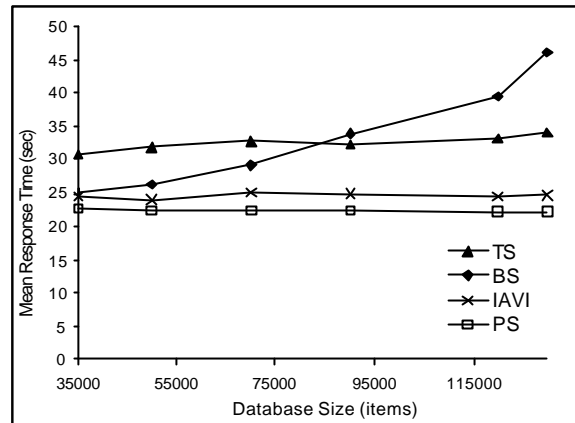
Figure 3: Mean Response Times vs Database Size
