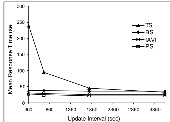
Figure 5: Mean Response Time vs Update Interval
