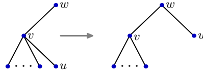
FIG. 4.1. Tree transformation 1
