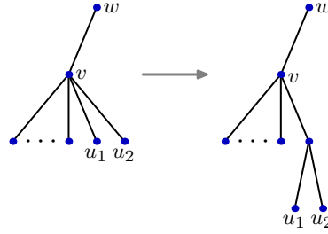
FIG. 4.2. Tree transformation 2
