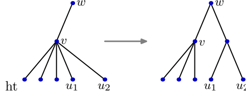
FIG. 4.3. Tree transformation 3
