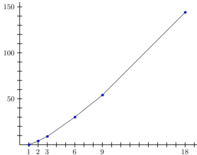
FIG. 6.2. Graph of \lambda^*(n)
