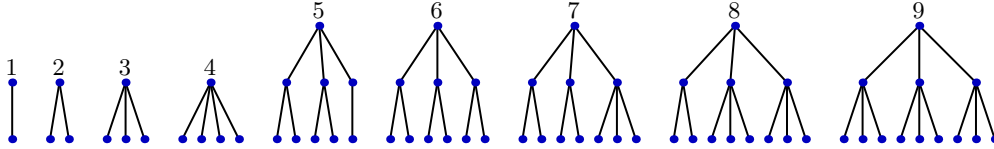
FIG. 6.1. Optimal small trees
