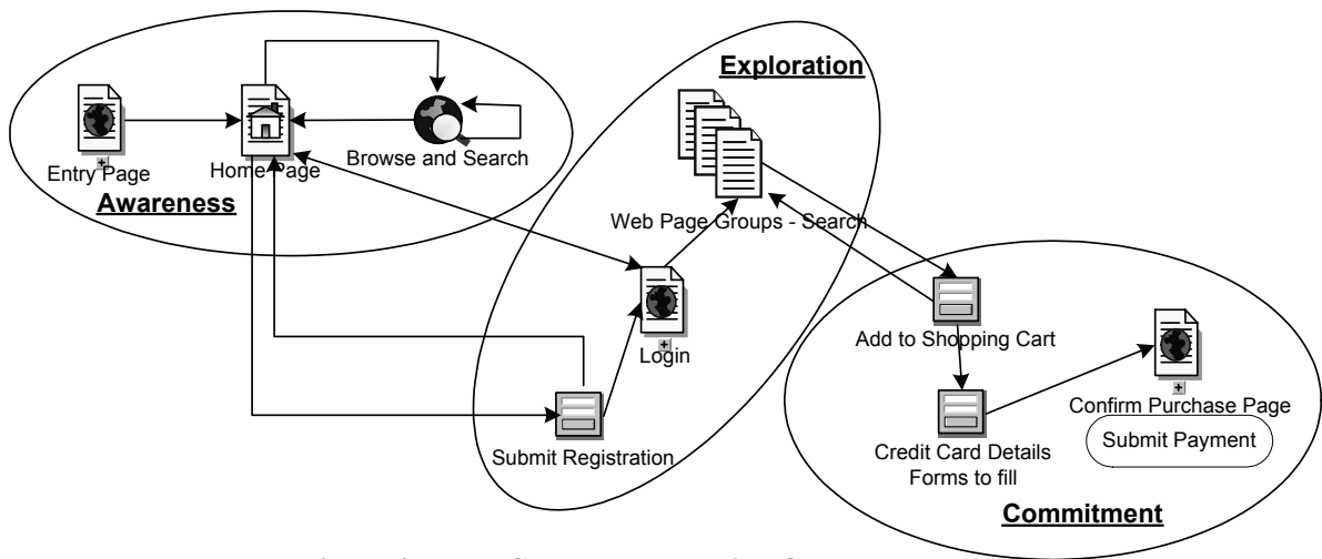
Figure 2 The e-Customer Behavior Graph
