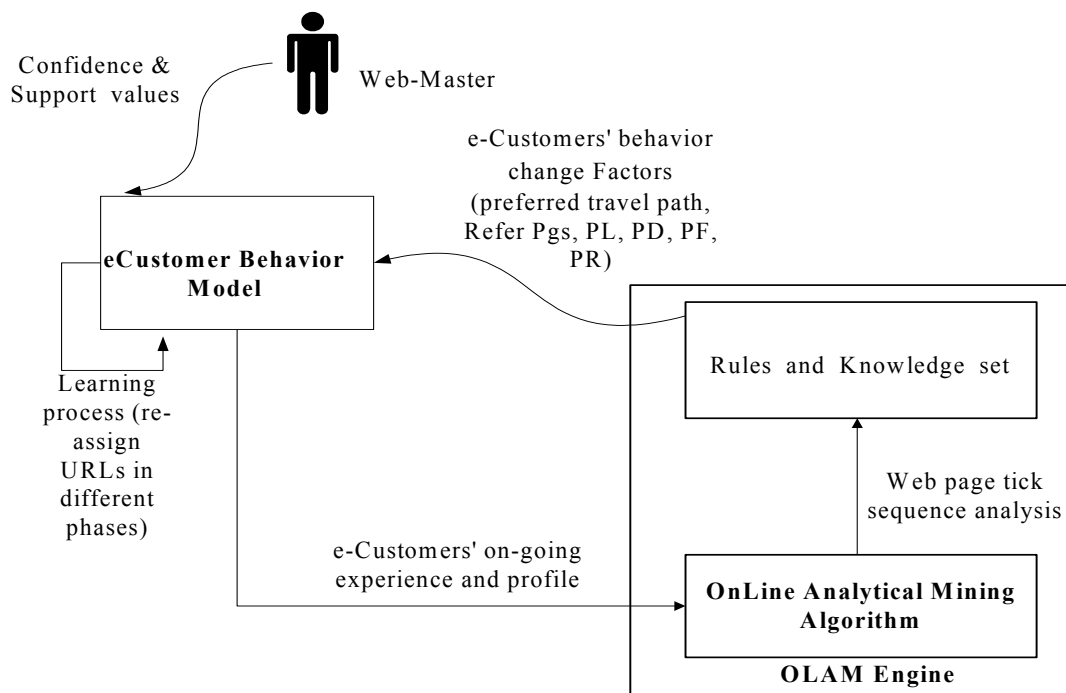
Figure 3 The OLAM Methodology for Internet Marketing Support
