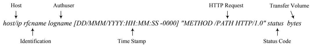
Figure 5 Common Log Format
