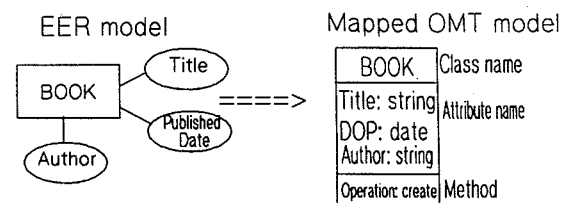
Figure 1 Map an entity to a class
