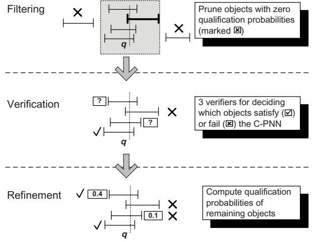
Fig. 3. Solution Framework of C-PNN.
