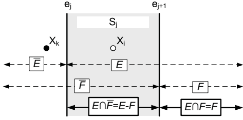
Fig. 15. Correctness proof of U-SR.
