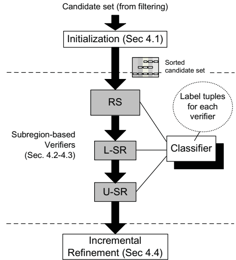
Fig. 5. The Verification Framework.
