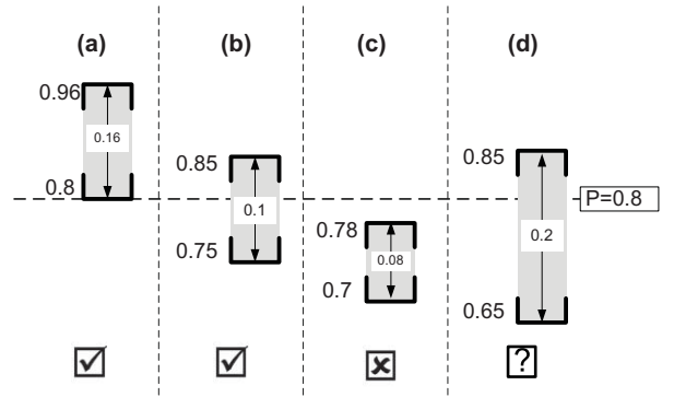
Fig. 4. C-PNN with P = 0.8 and \Delta = 0.15 .
